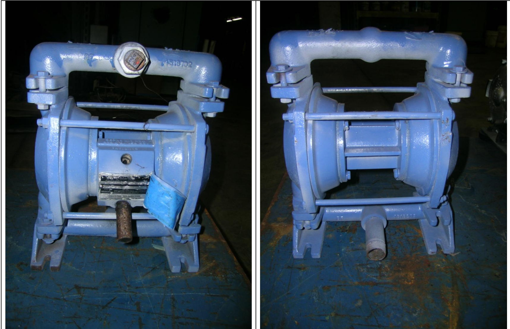
4) Pic no. 112 5EA ITT-MARLOW 1" air diaphragm pump Mod 0100A10 1AOD-CBBB ser 751473 1" inlet/outlet w air regulator, water trap& oiler
